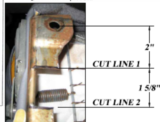
FIG. 2 SEAT FRAME MODIFICATION
