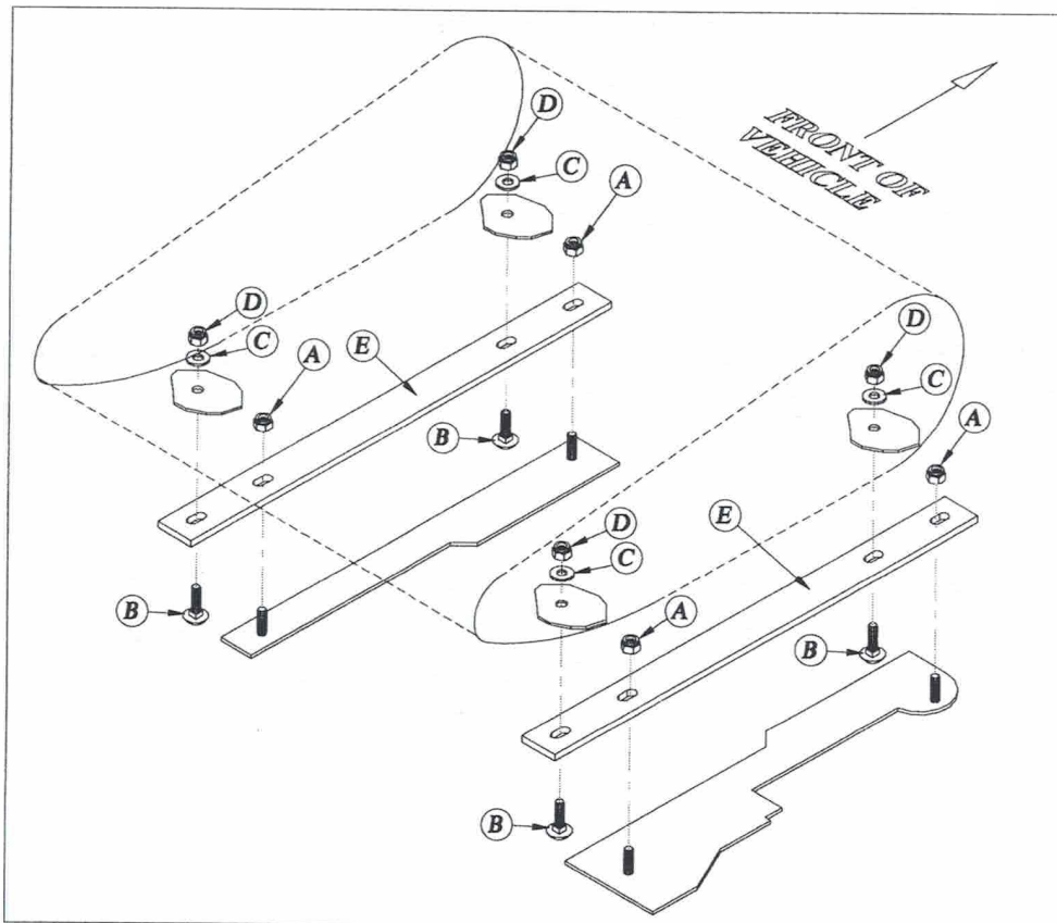
FIG. 1 DRIVER'S SIDE INSTALLATION
