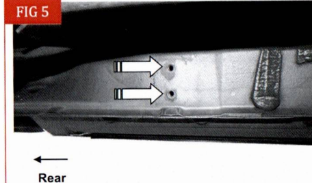
(Fig 5) Driver/Left rear mounting location
