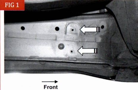
(Fig 1) Driver/Left front mounting location.
