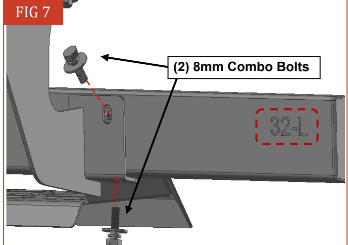
(Fig 7) Attach Running Board to the Mounting Brackets
