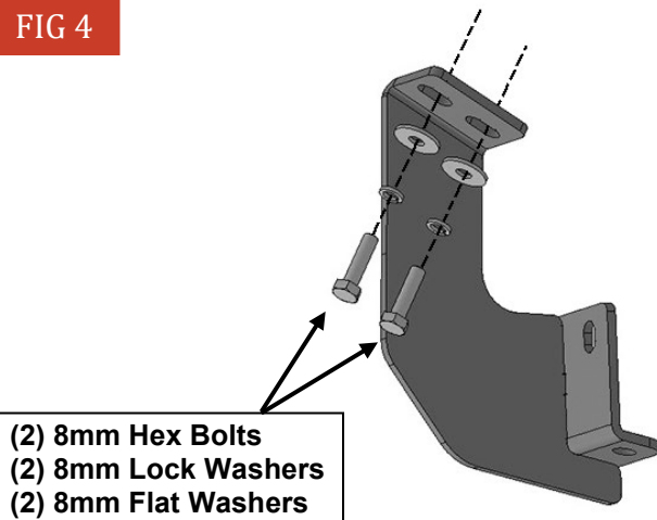
(Fig 4) Attach Driver/Left Center & Rear Mounting Bracket to the floor panel
