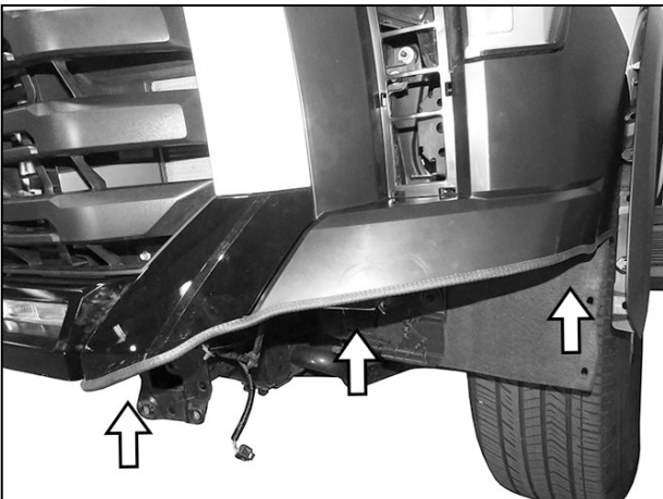
(Fig 43) Temporarily install Bumper (see Figures 48 and 49). Check fit between Bumper and trim plastic as necessary. Clean up cut sections and push Edge Trim onto cut bumper covers and fill panels (arrows)
