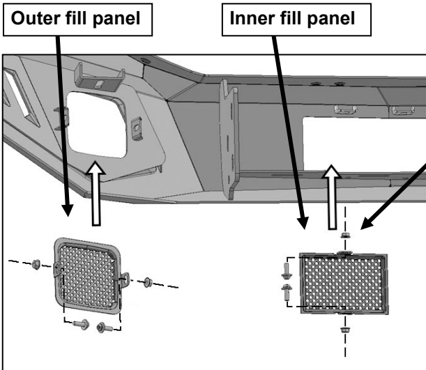
(Fig 45) Attach Mesh Fill Panels as desired to fill unused openings for lights (lights not included)
