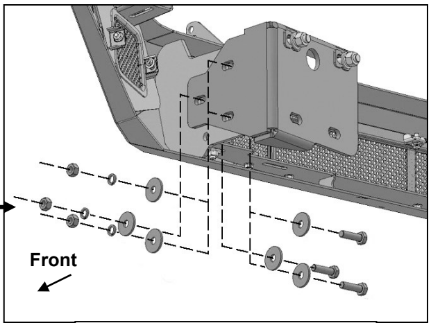
(Fig 48) Attach Bumper to inside of driver/left side Frame Bracket
