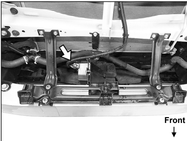
(Fig 8) Unplug active air dam motor (arrow)
