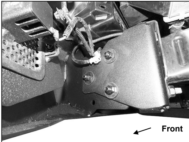
(Fig 49) Driver/left side of Bumper installation pictured from below
