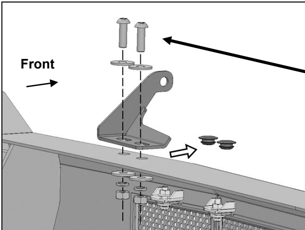
(Fig 47) Remove rubber plugs to attach Top Light Bracket to Bumper
