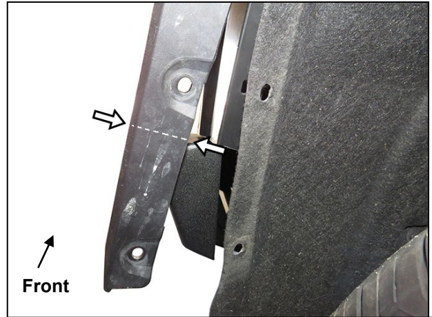
(Fig 50) Cut end of fender flares to match Bumper. Reattach fender flare and fender liner
