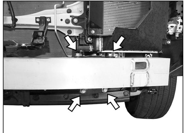
(Fig 9) Remove aluminum impact bumper from end of frame (arrows-driver/left side pictured)
