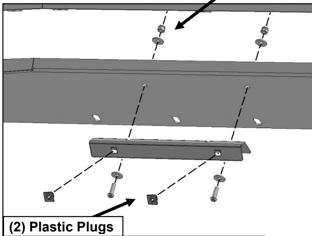
(Fig 51) Attach License Plate Bracket to Front Bumper
