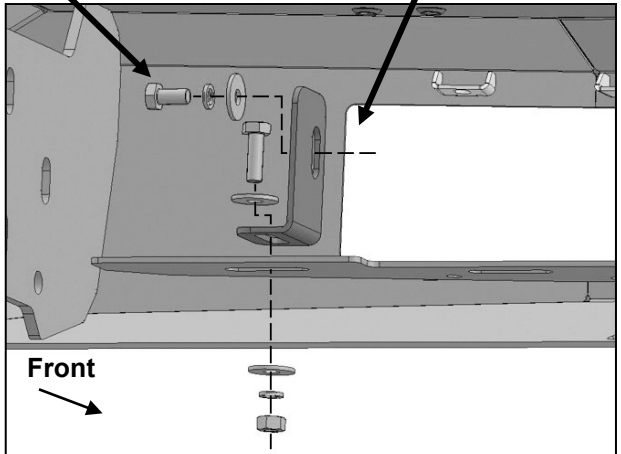
(Fig 46) Bracket illustration is a suggestion only. Brackets are offset to allow adjustment for all widths of lights
