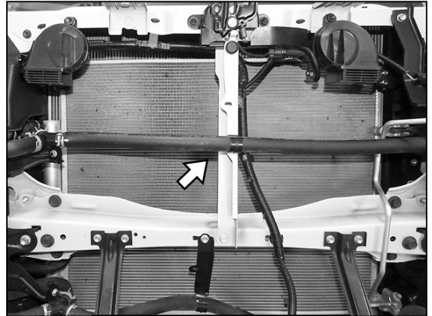
(Fig 19) Release hose from center support (arrow)
