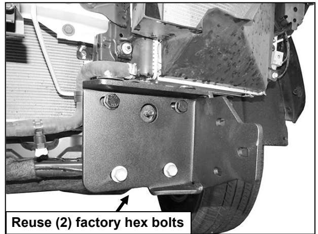
(Fig 30) Driver/left Mounting Bracket installed
