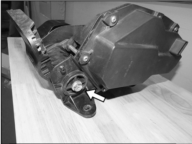
(Fig 13) Remove long pivot bolt (arrow)
