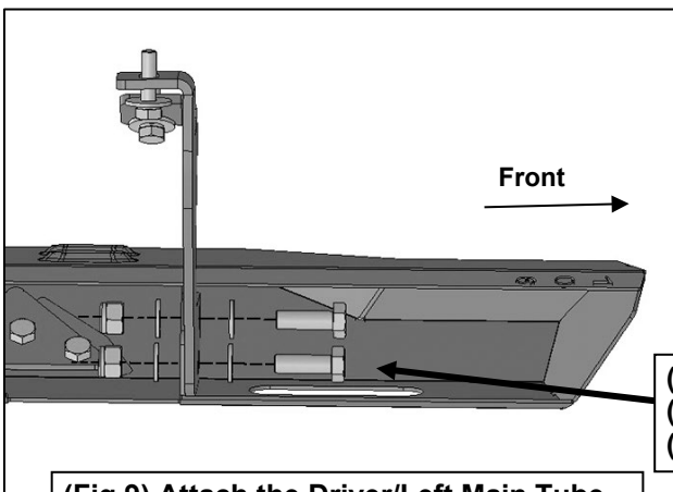
(Fig 9) Attach the Driver/Left Main Tube to the Mounting Brackets
