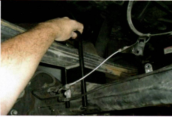
Slide new u-bolts over leaf pack and bump stop bracket.
