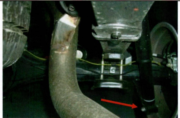
Remove rear lower shock bolt and disconnect shock.
