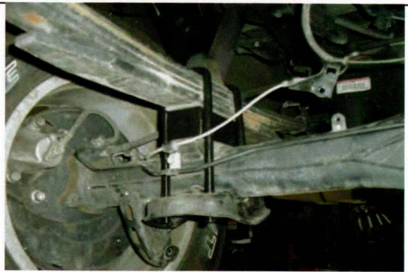
Attach lower mounting plate with provided hardware.
