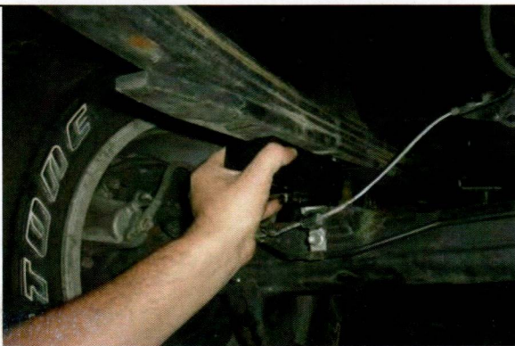
Place new lift block into position between axle and leaf pack.
