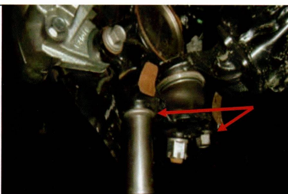
Remove (2) lower ball joint mounting bolts
