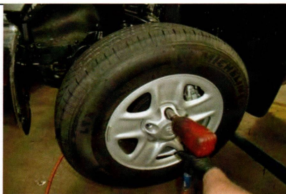
Remove front wheels/tires
