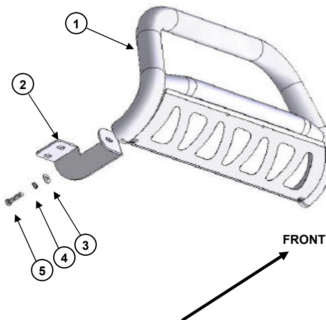
Image 1. Passenger side bracket.
