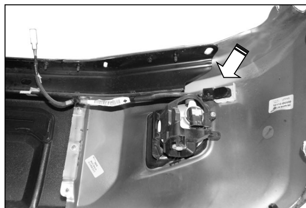
(Fig 18) Slide white plastic cover off sensor. Unplug wire harness. Remove Sensor.
