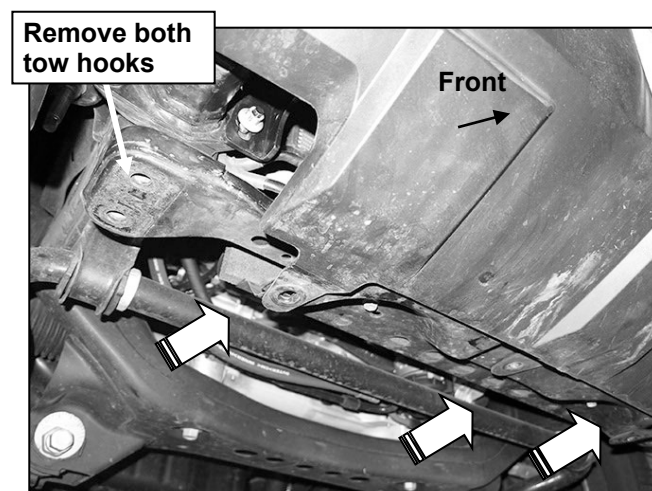
(Fig 6) Remove hardware attaching plastic cover on bottom of bumper to cross member (arrows)
