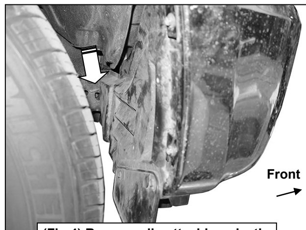
(Fig 4) Remove clip attaching plastic cover to side of frame (arrow)
