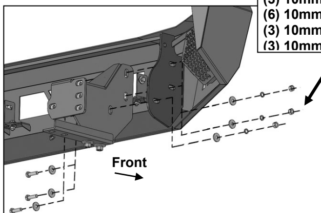
(Fig 15) Front Bumper attached to Passenger side Frame Bracket illustrated
