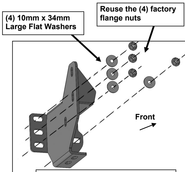
(Fig 9) Passenger/right side Frame Bracket attached to frame
