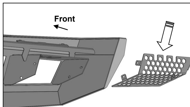
(Fig 14) Remove screens if necessary for clearance/access to outer light mounts
