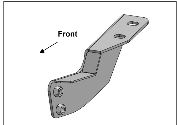
(Fig 8A) Passenger side Frame Mounting Bracket
