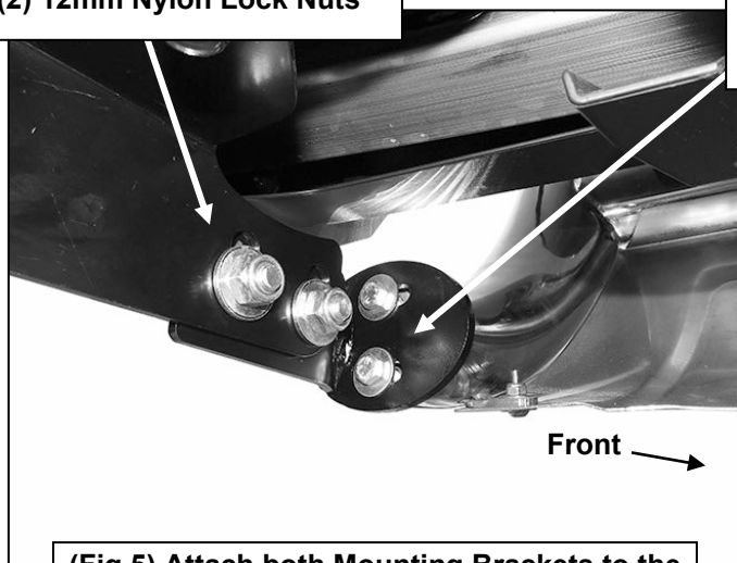
(Fig 5) Attach both Mounting Brackets to the ends of the Bull Bar first, then attach the Bull Bar and Brackets to the Frame Brackets
