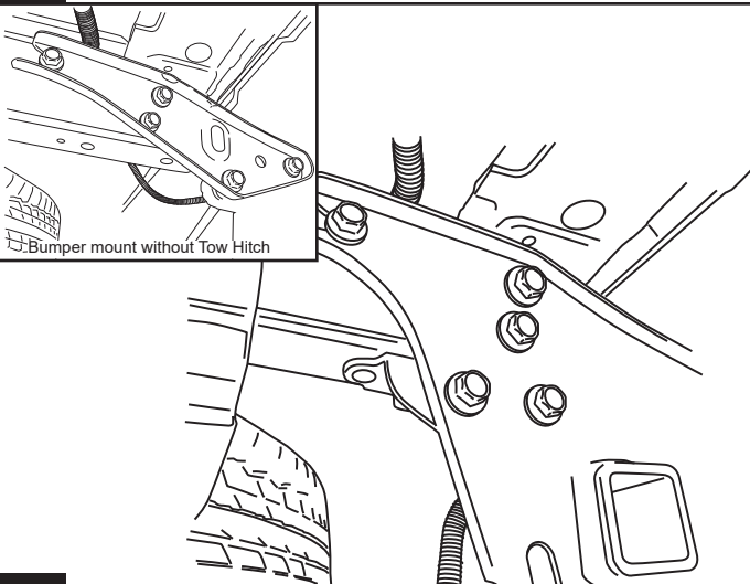
Bumper Mount with Tow Hitch
