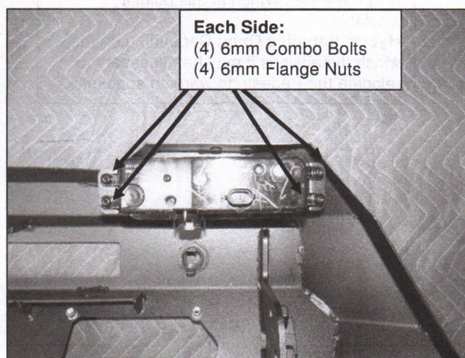
(Fig 53) Install Factory Fog Lights onto Fog Light Housing using indicated hardware.
