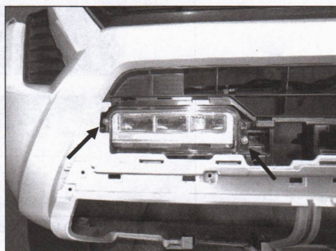
(Fig 31) From front side, remove fog lights.
