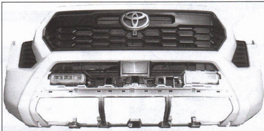
(Fig 25) Upper and lower front bumper plastic removed
