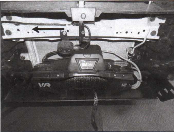
(Fig 48) Install Winch at this point if available. Hybrid Vehicles Only: Depending on the winch dimensions it may be necessary to relocate the Pedestrian warning speaker
