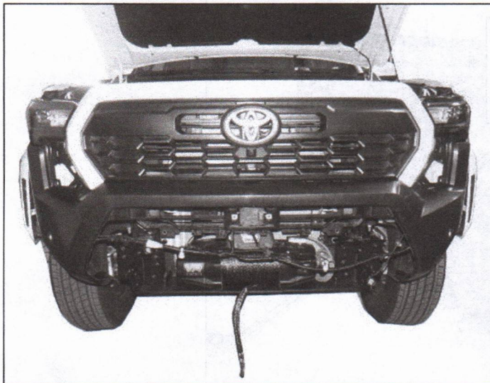
(Fig 50) Carefully reinstall the Front Clip onto the vehicle. Make sure all clips go into their original latch points and wire harness is not caught between any choking points.
