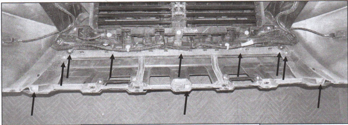
(Fig 22) Locate and remove 10 small screws holding the panels.
