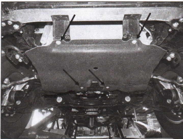
(Fig 15) Remove splash guard.
