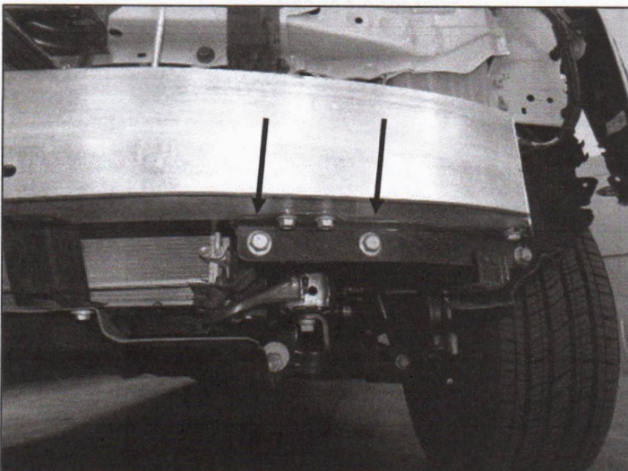
(Fig 17) Remove two lower frame horn bolts from crash bar. Repeat Steps 15-16 for Passenger Side, and fully remove crash bar.
