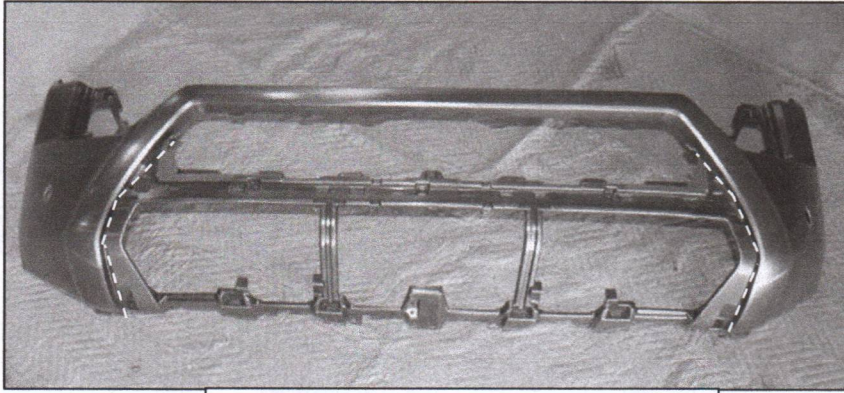
(Fig 36) Trim lower section of front clip under guide lines. Bumper disassembled for illustrative purposes only
