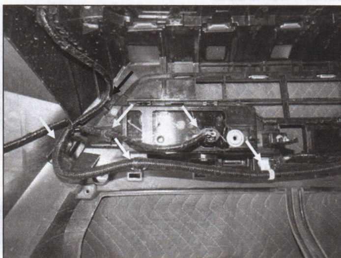
(Fig 28) On Left fog light area, unfasten indicated clips and unplug fog light. Repeat for Right fog light.
