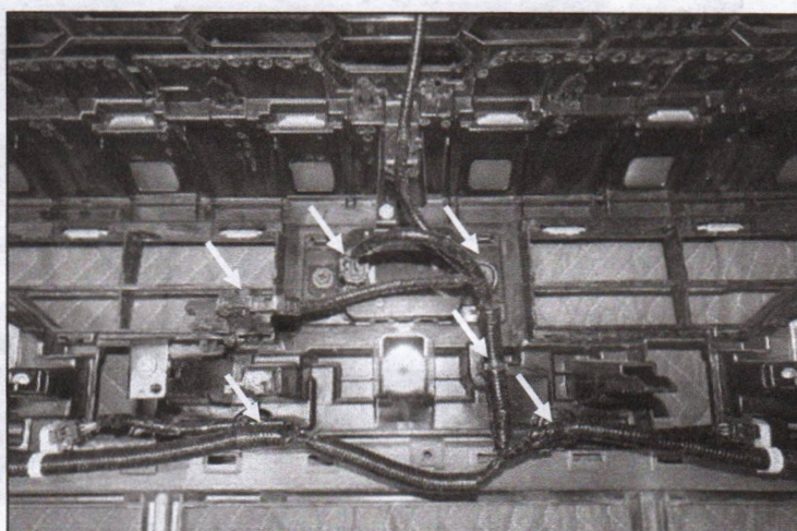
(Fig 29) Unfasten indicated clips in the center and unplug TSS module
