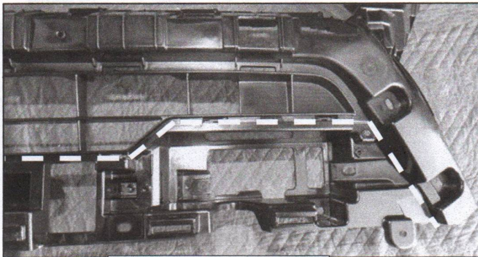
(Fig 33) Cut along the edge on the side and under the grille opening
