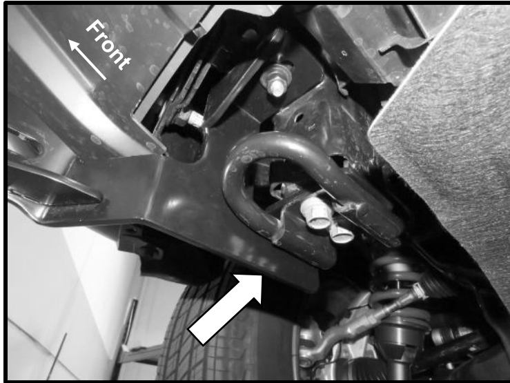
(Fig 5) For optional tow hook re-installation, stack them underneath the Mounting Brackets as shown. Then re-use the OEM hardware to install both the mounting bracket and the tow hook to the mount point.
