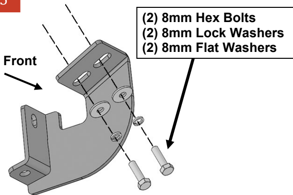
(Fig 5) Attach Driver/Left Center/Rear Mounting Brackets to the center and rear mounting locations
