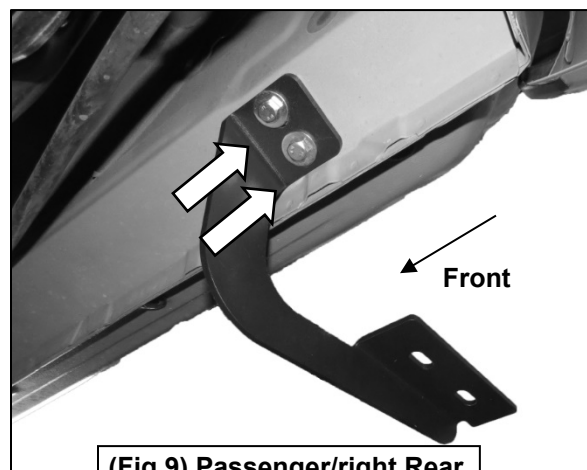
(Fig 9) Passenger/right Rear Mounting Bracket installed
