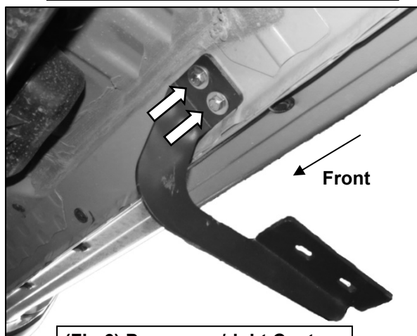
(Fig 6) Passenger/right Center Mounting Bracket installed
