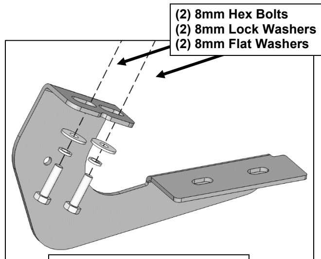
(Fig 5) Attach Passenger/right Center Mounting Bracket
