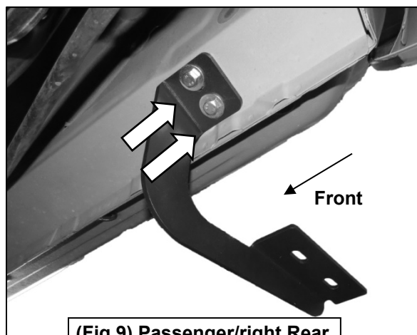
(Fig 9) Passenger/right Rear Mounting Bracket installed
