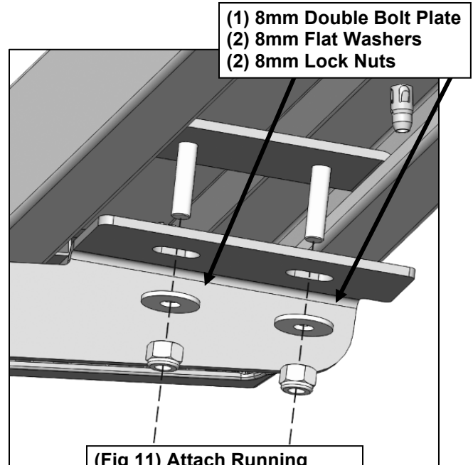
(Fig 11) Attach Running Board to Mounting Brackets
