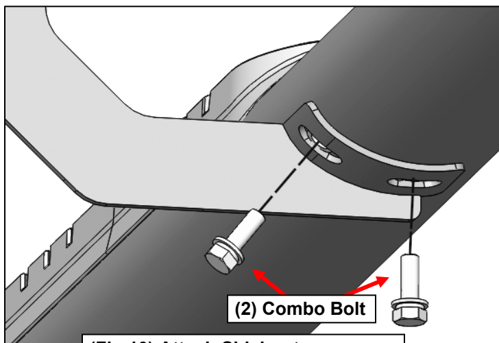
(Fig 10) Attach Sidebar to Mounting Brackets until hand tight
