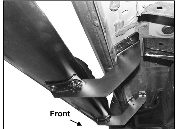
(Fig 10) Driver/left Side Bar attached to center Mounting Bracket
