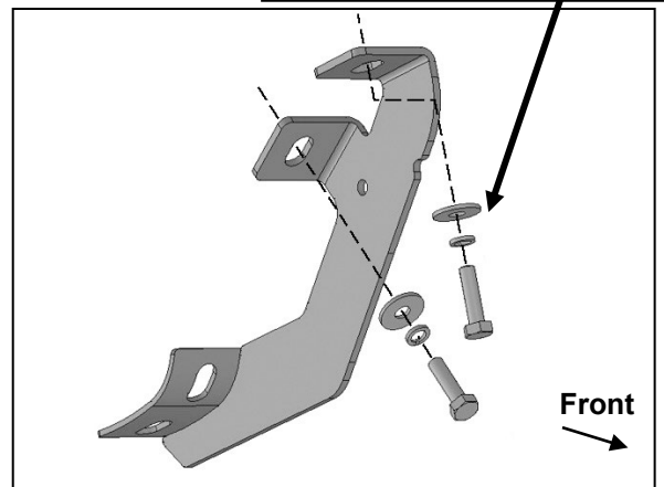
(Fig 2) Attach driver/left front Mounting Bracket to front location
