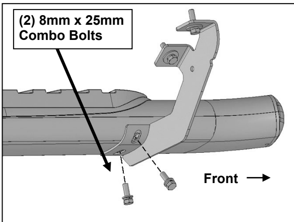
(Fig 7) Attach driver/left Side Bar to front Mounting Bracket
