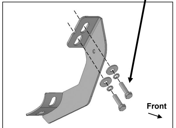
(Fig 4) Attach driver/left Center/rear Mounting Brackets
