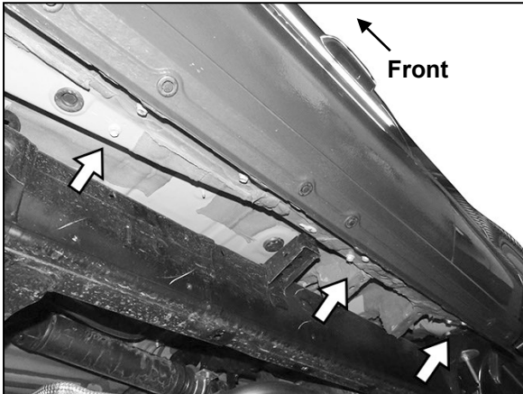
(Fig 1) Driver/left side mounting locations (arrows). Remove factory hex bolts from threaded holes as pictured
