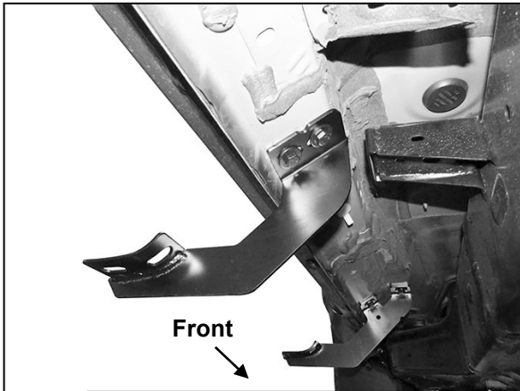
(Fig 5) Driver/left center Mounting Bracket installed
