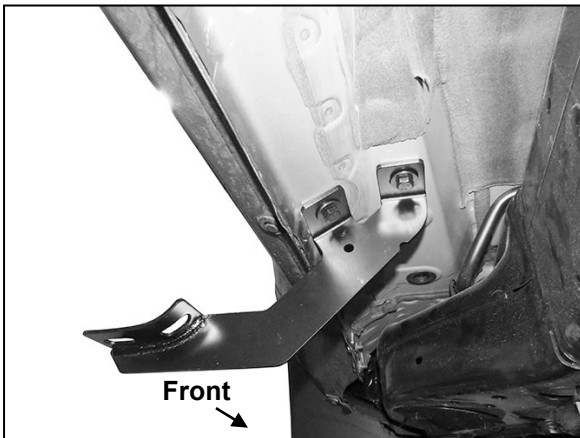
(Fig 3) Driver/left front Mounting Bracket installed
