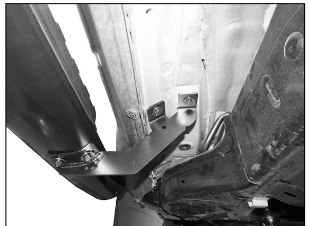
(Fig 8) Driver/left Side Bar front Bracket complete installation
