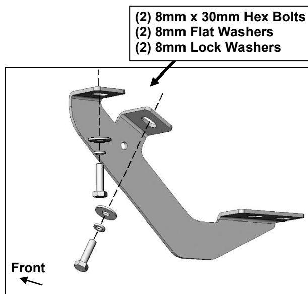
(Fig 2) Attach passenger/right front Mounting Bracket to front location
