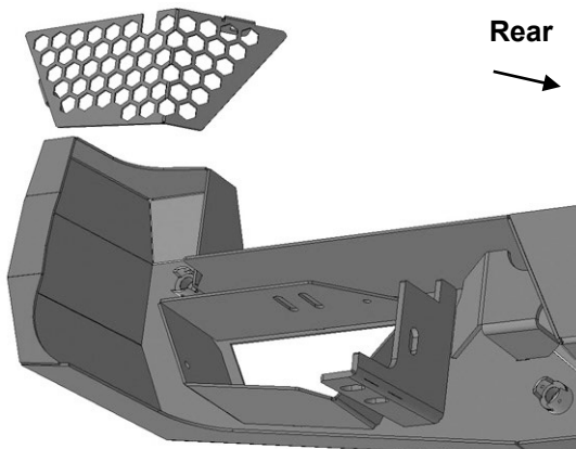
(Fig 3) Models with receiver hitch, remove the hex bolts attaching bumper to top of hitch
