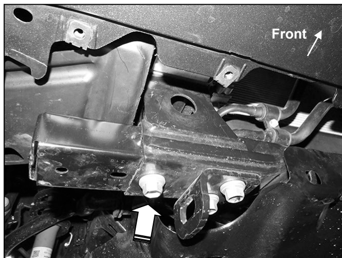
(Fig 2) Remove factory hex bolt (arrow)
