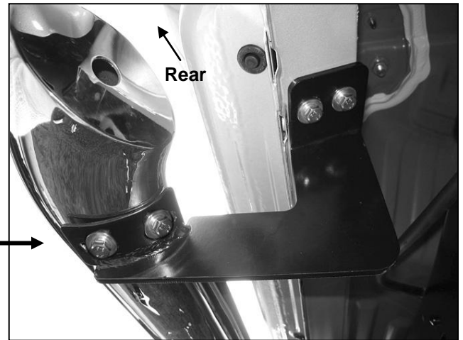
(Fig 4) Driver side rear mounting location pictured
