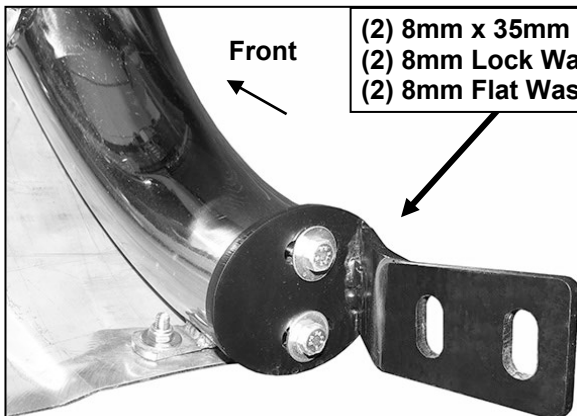
(Fig 11) Passenger side tube Mounting Bracket
