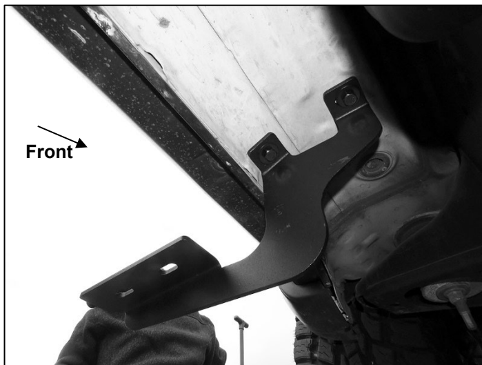
(Fig 3) Front Mounting Bracket attached to the front location
