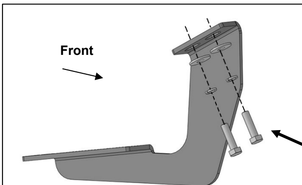
(Fig 5) Attach (1) Center/Rear Mounting
