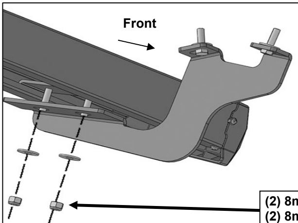
(Fig 10) Attach the Running Board to the front face of the Mounting Brackets
