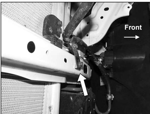
(Fig 7) Reuse hex bolt to attach bracket and Wedge to crossmember
