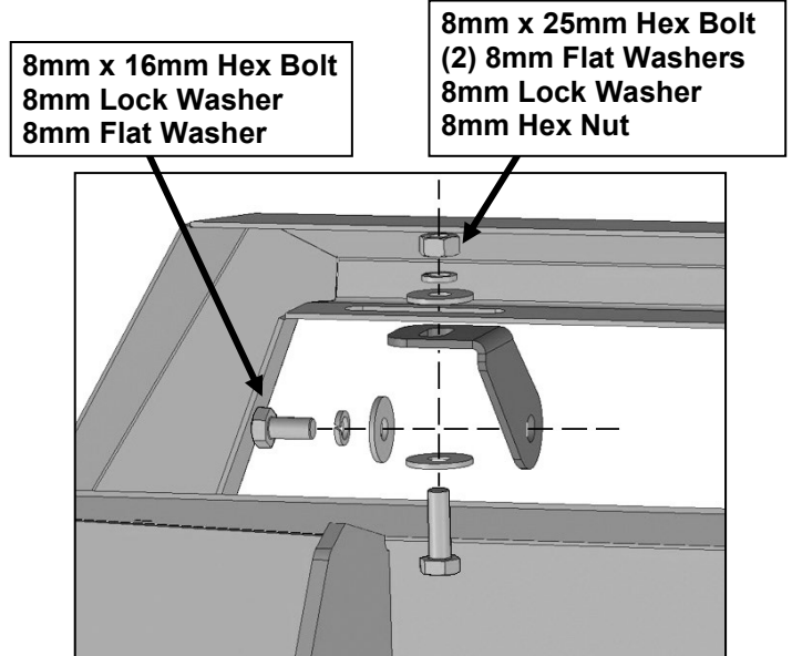
(Fig 21) Driver/left Top Light Bracket installed
