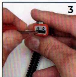
USE FLAT HEAD TO DEPRESS CLIPS & RELEASE PINS
