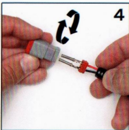
REMOVE TERMINALS FROM CONNECTOR & ROTATE 180°
