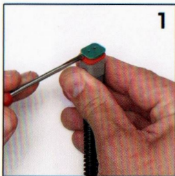
USE FLAT HEAD SCREW- DRIVER TO REMOVE CAP
