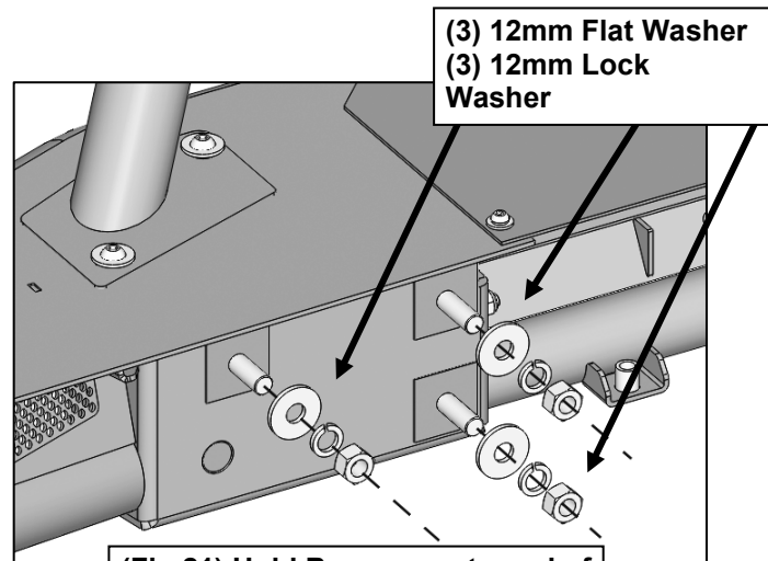
(Fig 21) Hold Bumper up to end of frame. Guide Bolt Plates in Bumper through threaded inserts
