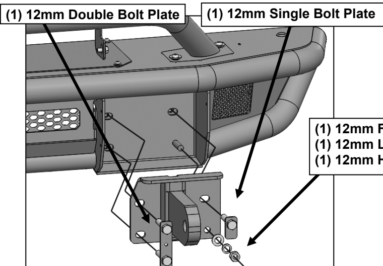
(Fig 18) Attach Shackle Mount to threaded stud on Bumper. Insert Single Bolt Plate through top inner mounting slot and Double Bolt Plate on the other side
