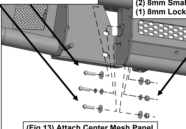
(Fig 13) Attach Center Mesh Panel with lightbar (not included)
