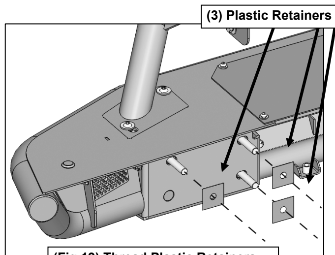
(Fig 19) Thread Plastic Retainers onto both Bolt Plates to hold them in place for Bumper installation
