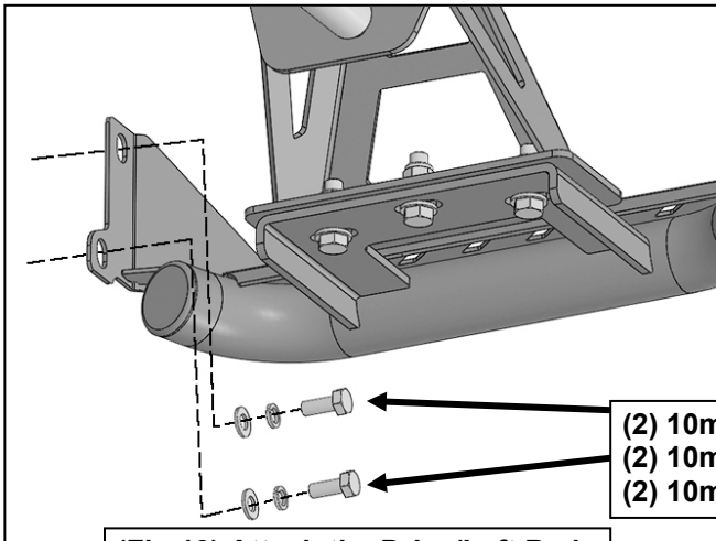
(Fig 13) Attach the Drive/Left Bed Guard assembly to the bumper
