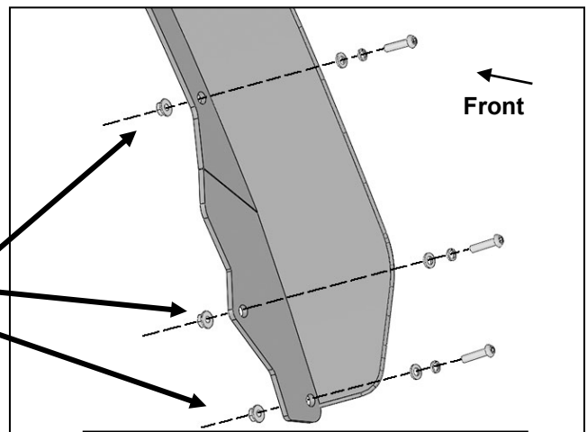
(Fig 9) Attach the Driver/Left Fender to the rear of the fender location
