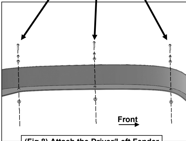
(Fig 8) Attach the Driver/Left Fender to the top of the fender location
