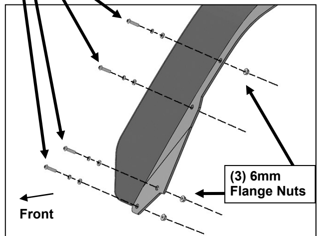
(Fig 7) Attach the Driver/Left Fender to the front of the fender location
