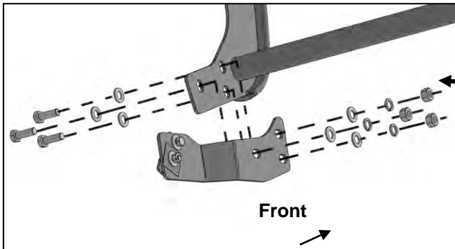
(Fig 10) Attach Grille Guard to the outside of the Driver/left side Mounting Bracket
