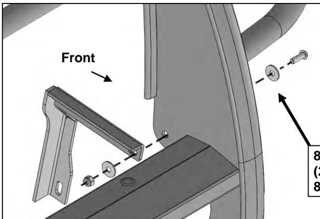
(Fig 12) Attach Grille Guard to the outside of the Driver/left Support Bracket
