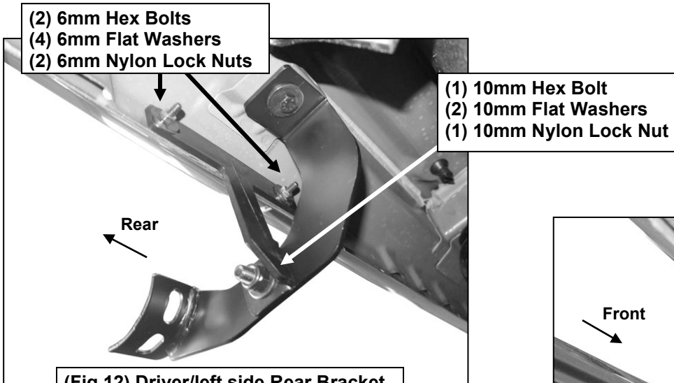
(Fig 12) Driver/left side Rear Bracket attached to Rear Support Bracket
