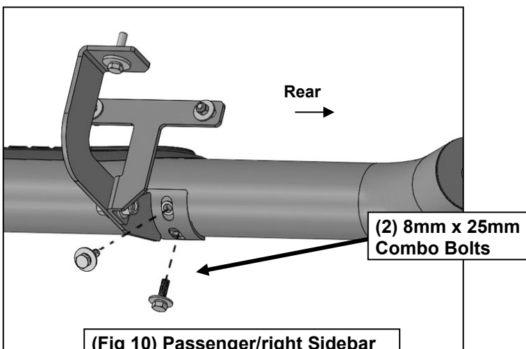
(Fig 10) Passenger/right Sidebar attached to rear Brackets
