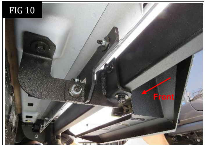
(Fig 10) Passenger/Right near mounting bracket and support bracket attached.
