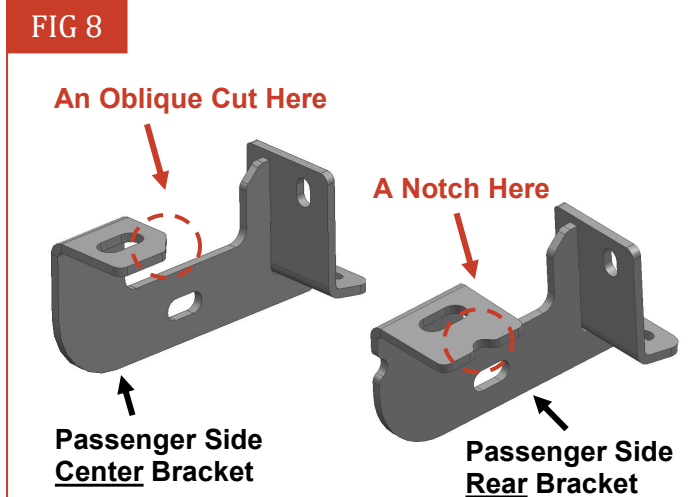
(Fig 8) The Center and Rear Mounting Brackets are similar but are unique
