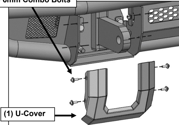
(4) 6mm Combo Bolts
