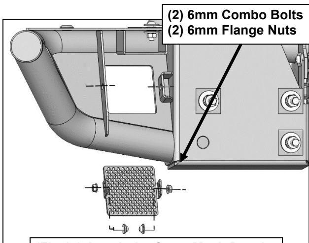
(Fig 15) Attach the Outer Mesh Panels to the tabs on the back of the Bumper
