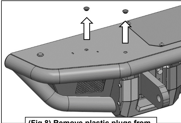
(Fig 8) Remove plastic plugs from BN Hoop installation points
