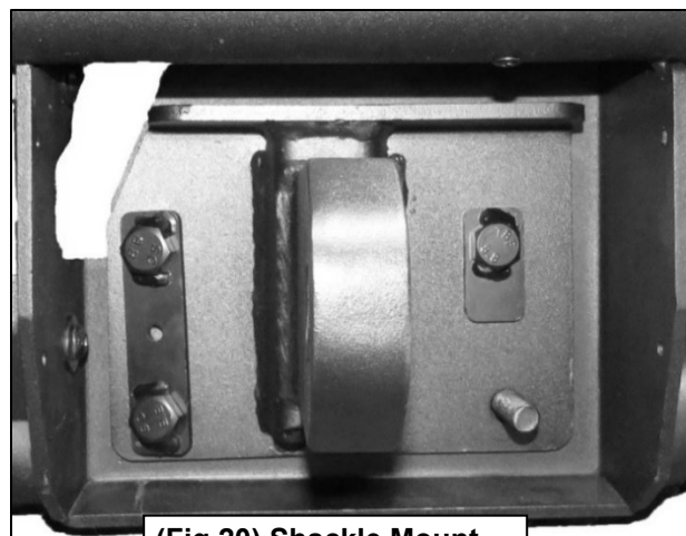
(Fig 20) Shackle Mount with Bolt Plates attached
