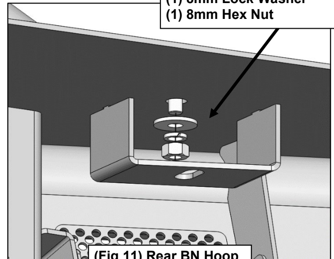
(Fig 11) Rear BN Hoop installation point
