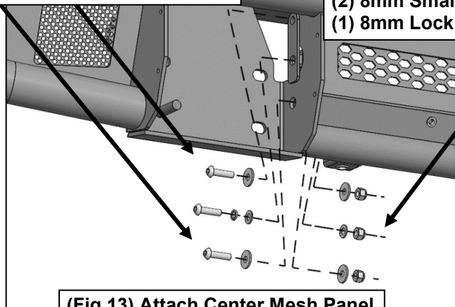
(Fig 13) Attach Center Mesh Panel with lightbar (not included)
