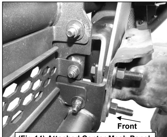
(Fig 14) Attached Center Mesh Panel
