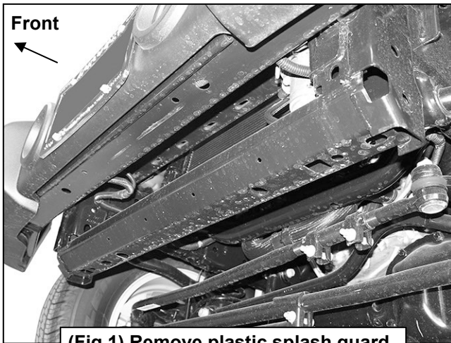
(Fig 1) Remove plastic splash guard or skid plate from bottom of bumper
