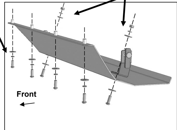
(Fig 8) Attach the top of the Skid Plate to the back of the Bumper. Attach the bottom of the Skid Plate to the Skid Plate Brackets, (JL/JT model installation illustrated)
