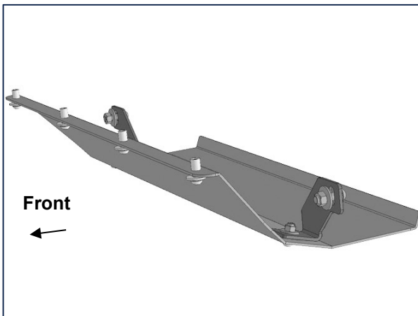
(Fig 9) Example of complete installation on JK model
