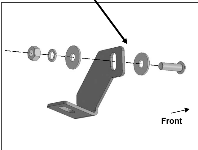
(Fig 3) JK models only, attach driver/left Skid Plate Bracket to the back of the crossbar
