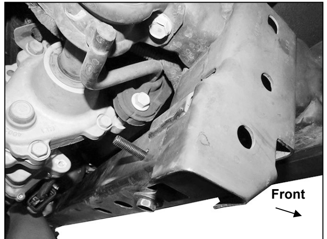
(Fig 2) Insert (1) 10mm x 35mm Button Head Bolt with (1) 10mm Flat Washer into and out the back of the crossbar (passenger/right side pictured)
