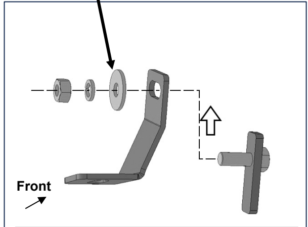
(Fig 6) JL/JT models, attach the driver/left Skid Plate Bracket to the 10mm Bolt Plate
