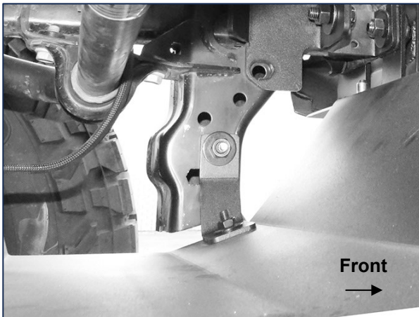
(Fig 7) Driver/left JL/JT mounting Bracket pictured installed with Skid Plate
