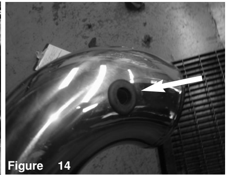
Figure 14 Install the grommet to the hole on the intake tube. This will be used for the temperature sensor.
