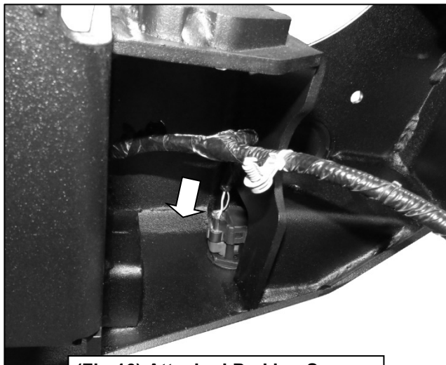
(Fig 16) Attached Parking Sensor
