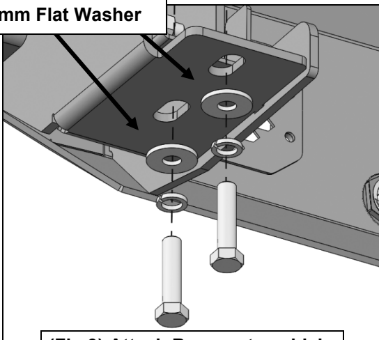
(Fig 9) Attach Bumper to vehicle using bottom mounting slots
