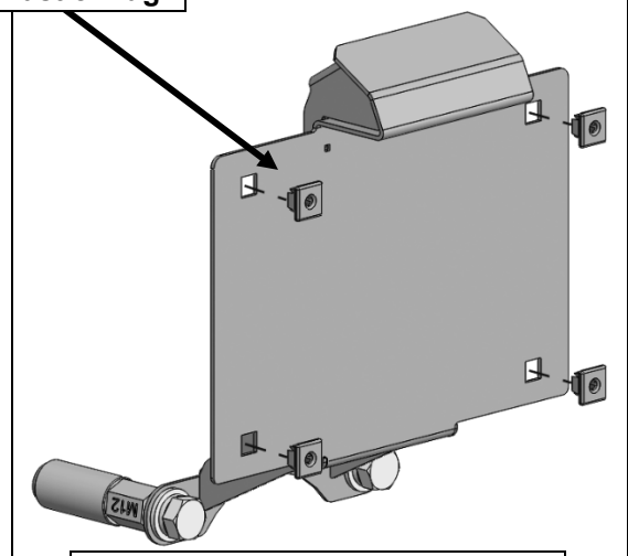
(Fig 20) Attach License Plate to License Plate Relocation Bracket
