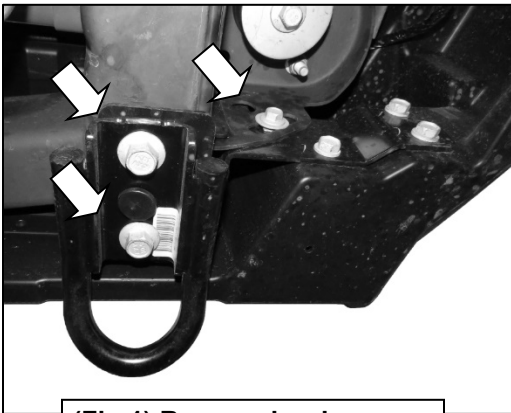
(Fig 1) Remove hardware from underneath tow hook
