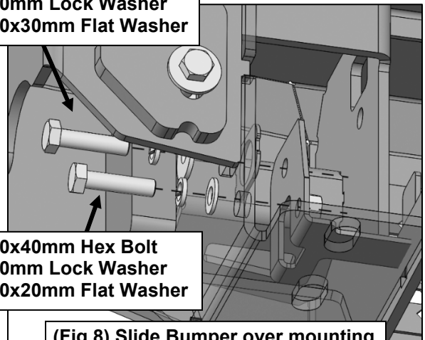
(Fig 8) Slide Bumper over mounting point then attach to Double Nut Plate using side mounting slots
