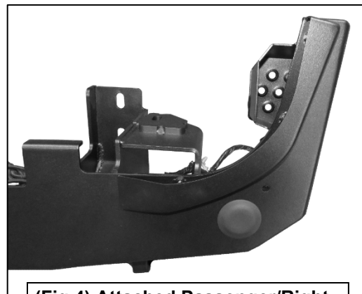
(Fig 4) Attached Passenger/Right Fill Panel on Bumper
