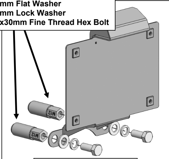
(Fig 19) Attach License Plate Relocation Bracket
