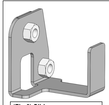
(Fig 6) Slide Passenger/Right Double Nut Plate into mounting slot
