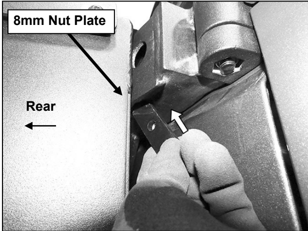
(Fig 3) Insert Nut Plate up and into top leg on Tire Mount
