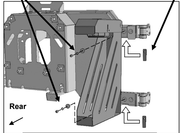
(Fig 4) Attach Water/Gas Container Tray to Nut Plates in tire mount
