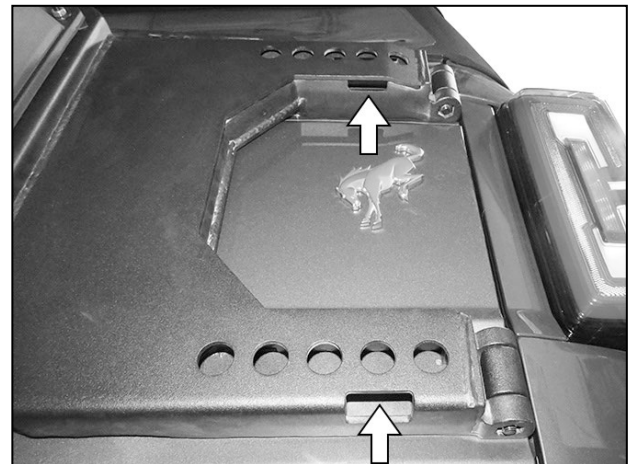
(Fig 2) Insert 8mm Nut Plates up into slots (arrows)
