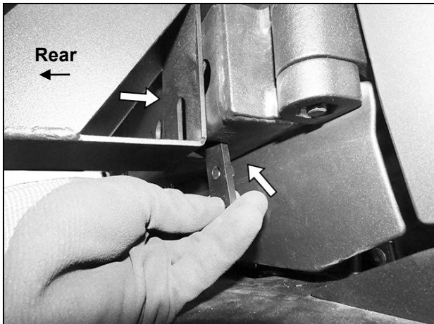
(Fig 5) Insert Nut Plate up into bottom leg on tire mount. Attach bottom of Water/Gas Container Tray to Nut Plate in tire mount (see Fig 4)
