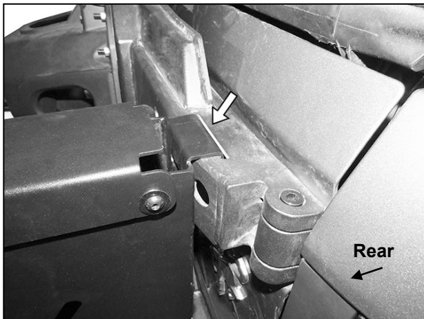
(Fig 1) Hang Water/Gas Container Tray from slot in top of tire mount
