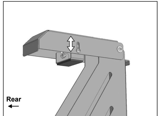
(Fig 6) Insert Water/Gas Container into the Tray. Adjust inner stop up or down to fit against Water/Gas Container and tighten hardware
